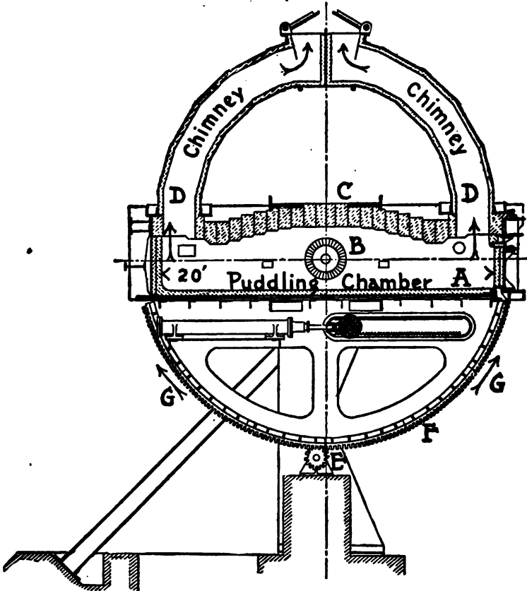
Fig. 121. Longitudinal Vertical Section of Roe's Rocking Puddling Furnace.
